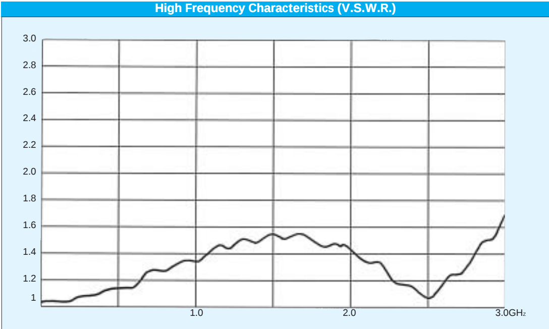
Note: Data taken using fully assembled and connected GT1-1S-HU and GT1-1P-DSA.
