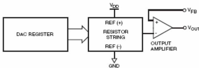
Figure 22. DAC Architecture
