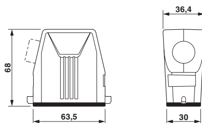
Dimensional drawing
