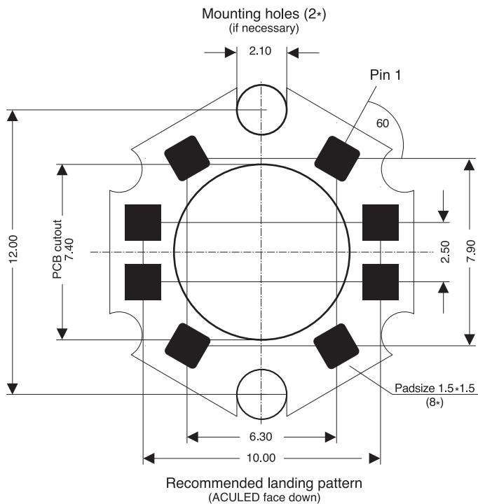
Recommended Solder Pad Geometry
