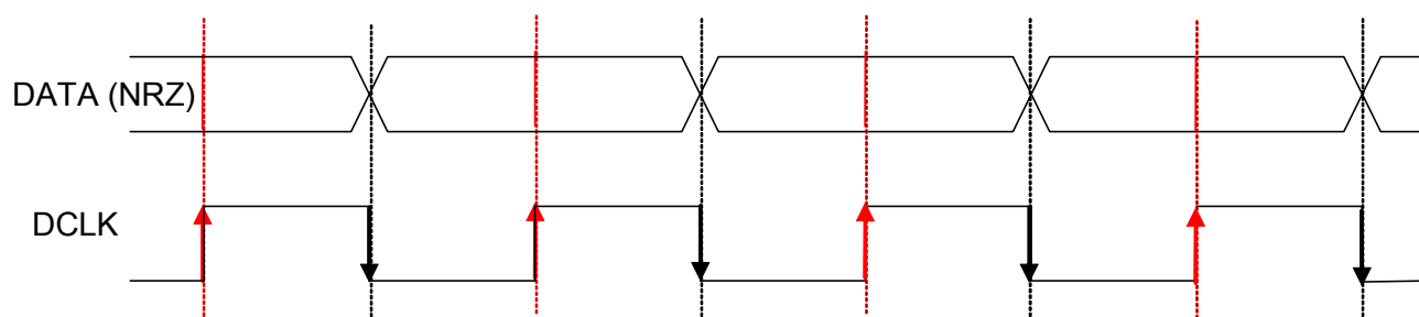
Figure 32. Rx Processing in Continuous Mode
