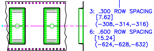
PACKAGE PARTS IN TAPE & REEL AS SHOWN (FIG 5)
