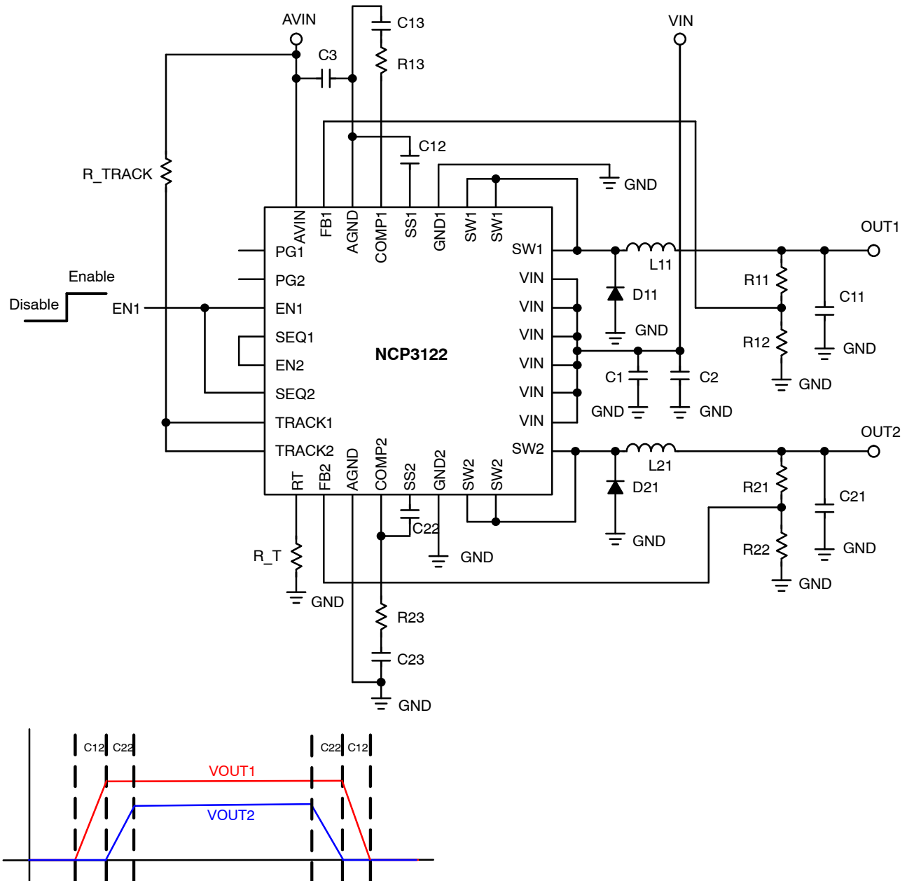
Figure 46. Sequential Configuration
