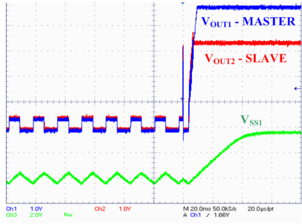
Figure 62. Master Voltage – End of OLM
