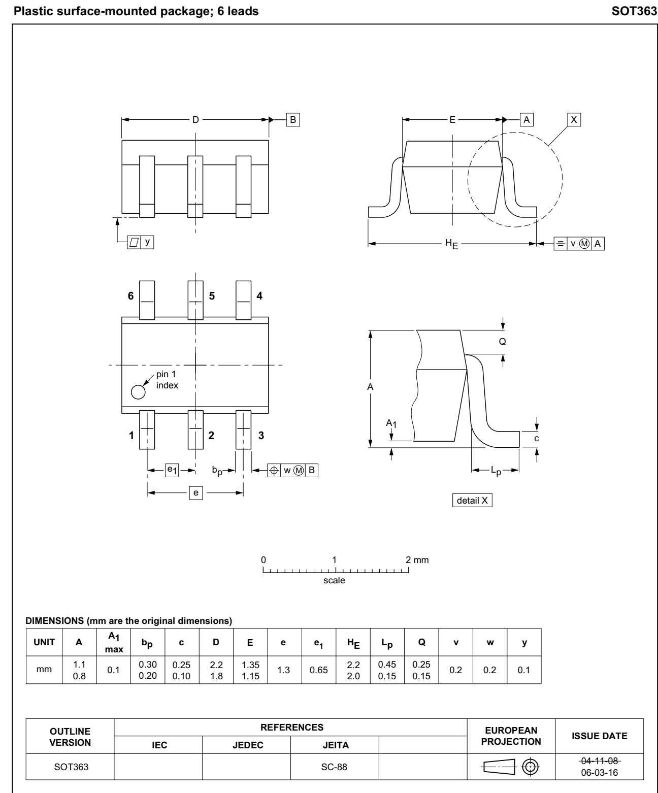
Fig 7. Package outline SOT363 (SC-88)
