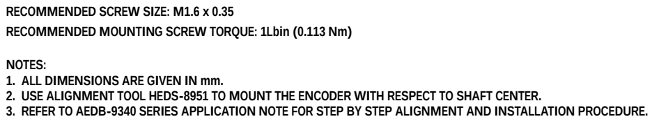
Figure 3b. 1024/2048 CPR encoder mounting considerations
