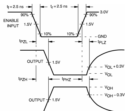
FIGURE 3. AC Waveforms
