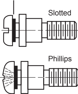
Self-Sealing Washers
