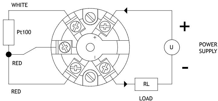
FIGURE 4 SEM203P CONNECTION DIAGRAM
