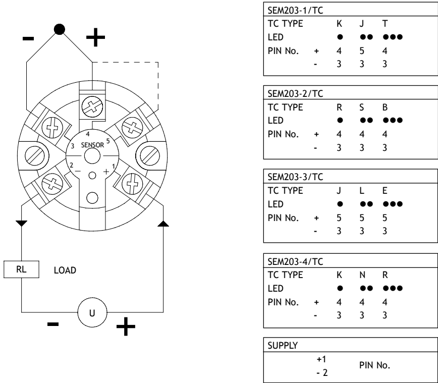
FIGURE 4 SEM203P CONNECTION DIAGRAM
