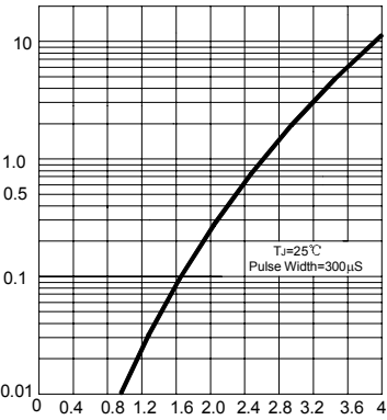
FIG.5 -- TYPICAL FORWARD CHARACTERISTIC
