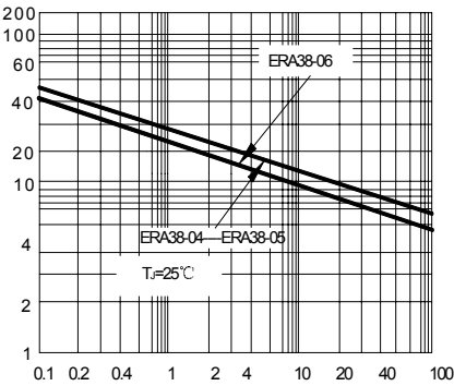
FIG.3--TYPICAL JUNCTION CAPACITANCE
