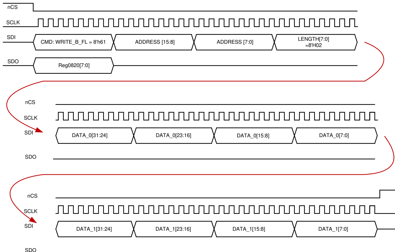
Figure 8-17. Write
