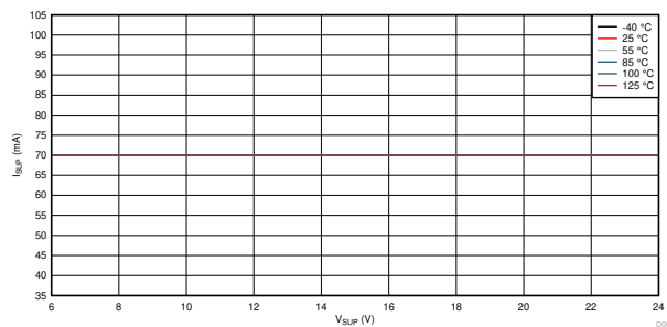
Figure 6-2. I_{SUP} Current Across Temperature and V_{SUP} LDO Output Only.
