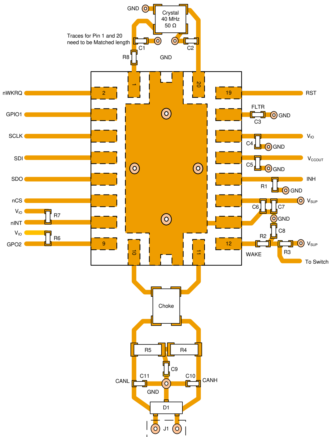
Figure 11-1. Example Layout
