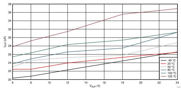
Figure 6-1. I_{SUP} vs V_{SUP} Sleep Mode
