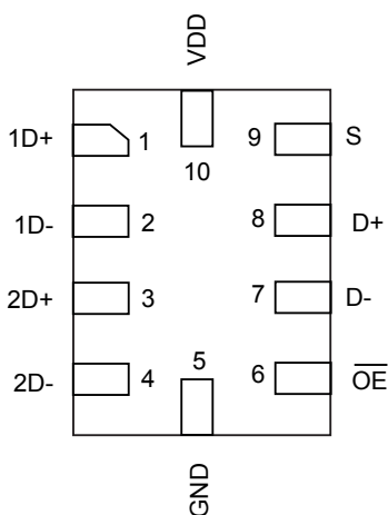
UQFN Package (Top View)
