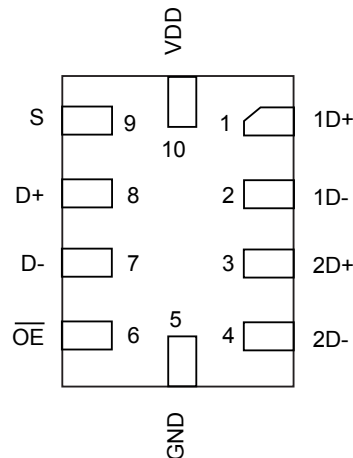
UQFN Package (Bottom View)
