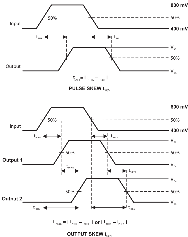
Figure 7. Skew Test
