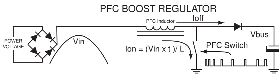
Figure 7-3. PFC Boost Regulator
