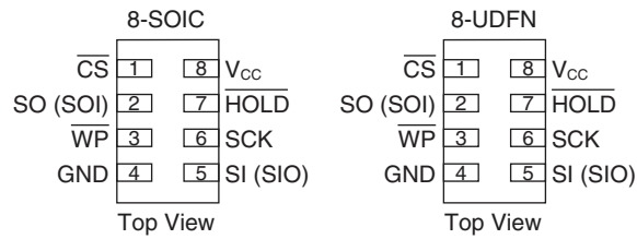
Figure 2-1. Pin Configurations
