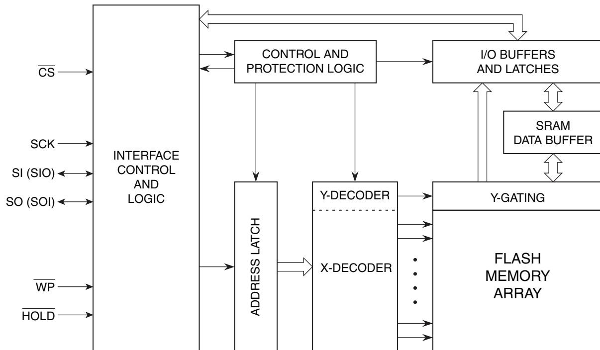
Figure 3-1. Block Diagram
