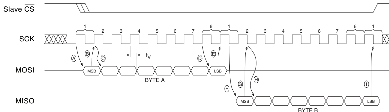
Figure 13-1. RapidS Operation
