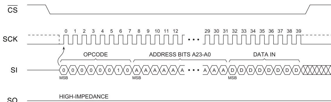
Figure 8-1. Byte Program
