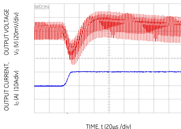
Figure 16. Transient Response to Dynamic Load Change from 50% to 100% at 12Vin, C_{out}= 2\text{x}47\mu\text{F} + 3\text{x}330\mu\text{F} , C_{Tune}=5600\text{pF} & R_{Tune}=220\text{ ohms}
