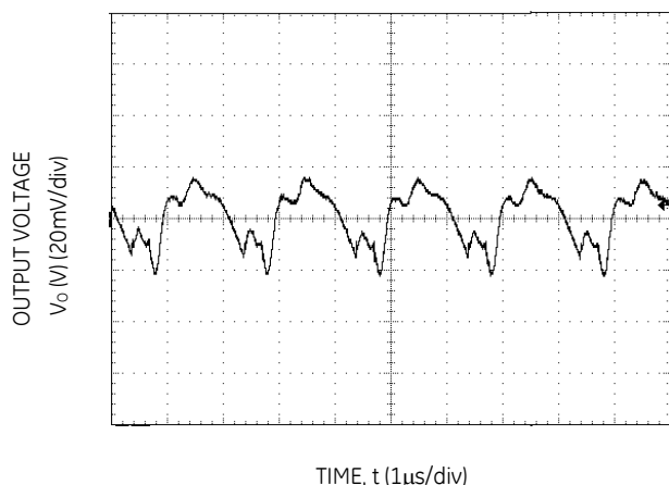
Figure 15. Typical output ripple and noise ( C_o=2\text{X}47\mu\text{F} ceramic, V_{IN} = 12\text{V} , I_o = I_{o,max} ).
