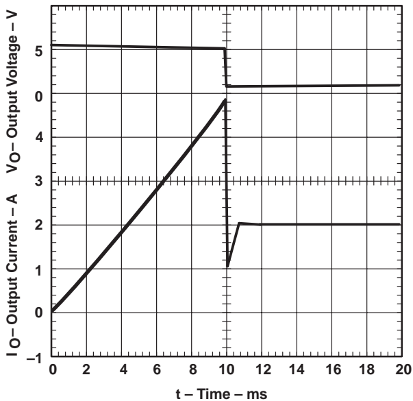
Figure 11. TPS2012 – Threshold Current, V_{I(IN)} = 5.5 V
