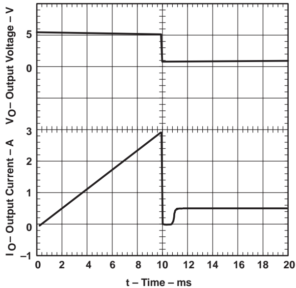
Figure 9. TPS2010 – Threshold Current, V_{I(IN)} = 5.5 V
