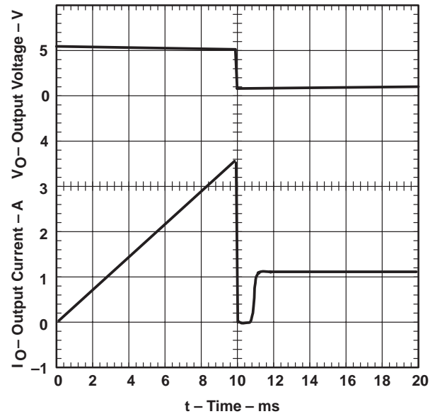
Figure 10. TPS2011 – Threshold Current, V_{I(IN)} = 5.5 V
