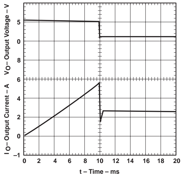
Figure 12. TPS2013 – Threshold Current, V_{I(IN)} = 5.5 V
