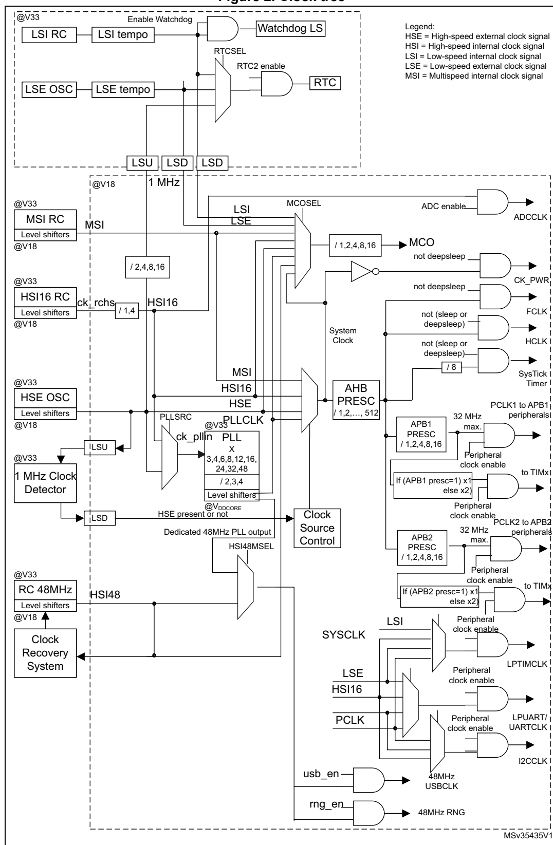
Figure 2. Clock tree
