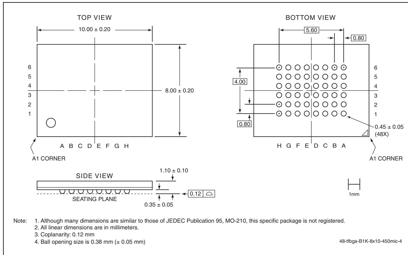
48-BALL THIN-PROFILE, FINE-PITCH BALL GRID ARRAY (TFBGA) 8MM X 10MM SST PACKAGE CODE: B1K
