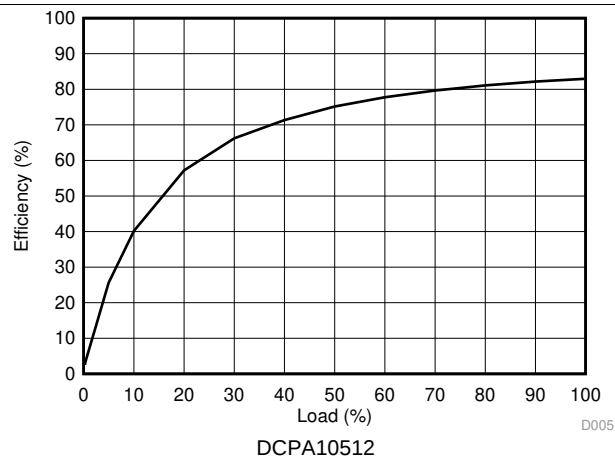
Figure 5. Efficiency versus Load
