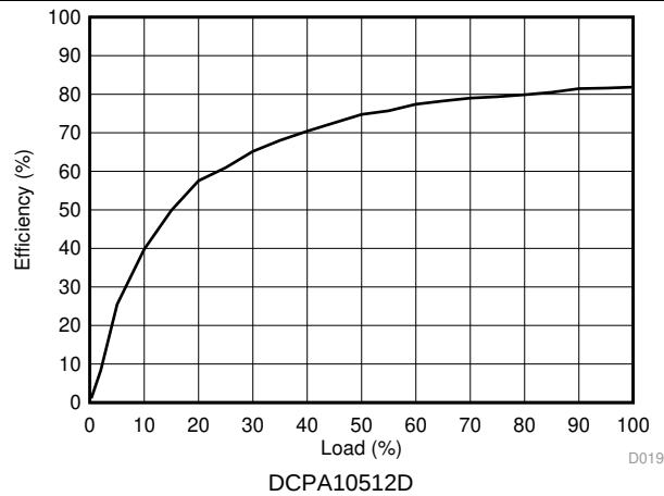
Figure 19. Efficiency versus Load
