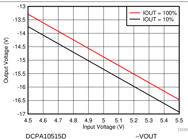
Figure 30. -VOUT Line Regulation
