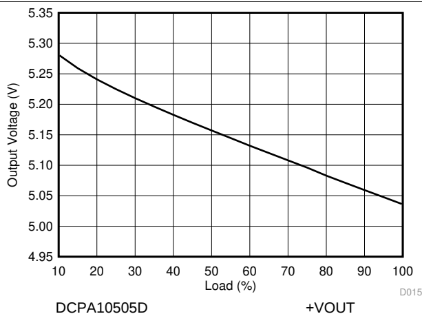
Figure 15. +VOUT Load Regulation
