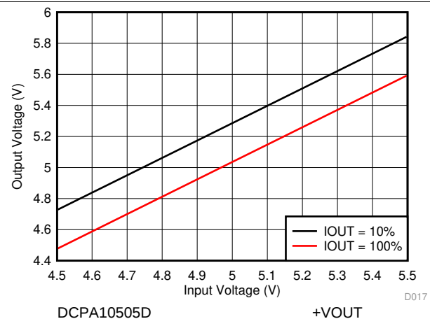
Figure 16. +VOUT Line Regulation
