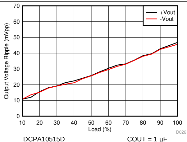
Figure 26. Output Ripple versus Load
