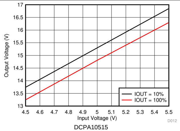
Figure 12. Line Regulation
