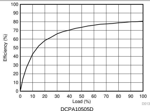
Figure 13. Efficiency versus Load
