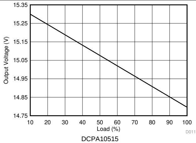
Figure 11. Load Regulation
