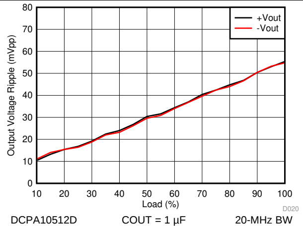
Figure 20. Output Ripple versus Load
