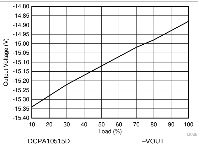
Figure 29. -VOUT Load Regulation
