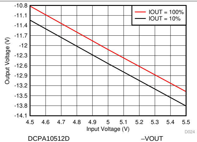
Figure 24. -VOUT Line Regulation
