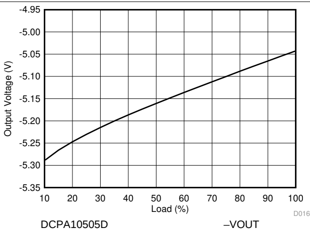
Figure 17. -VOUT Load Regulation
