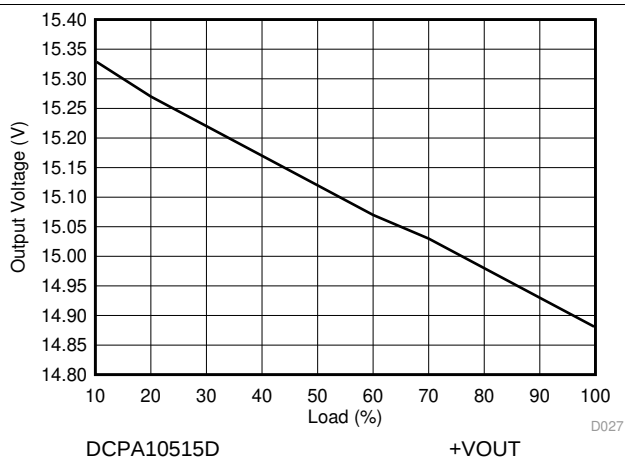
Figure 27. +VOUT Load Regulation
