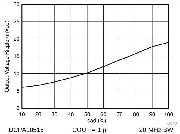
Figure 10. Output Ripple versus Load
