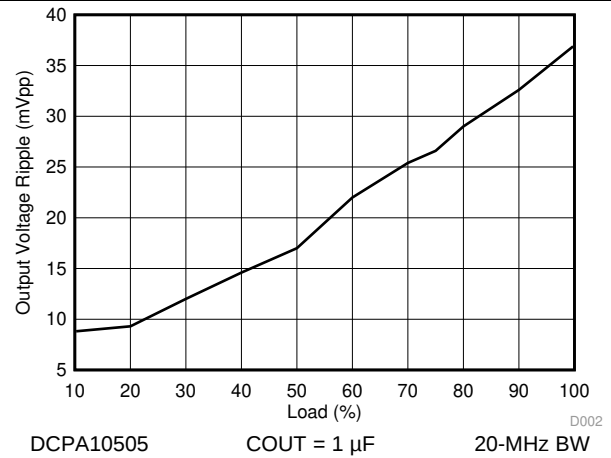
Figure 2. Output Ripple versus Load
