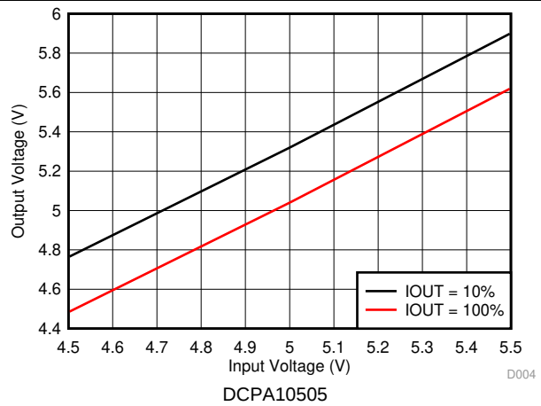
Figure 4. Line Regulation
