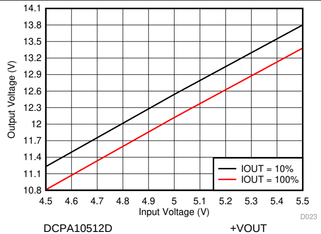
Figure 22. +VOUT Line Regulation
