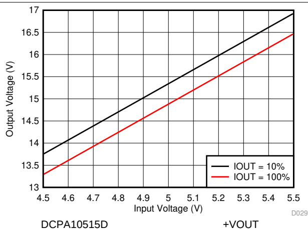
Figure 28. +VOUT Line Regulation
