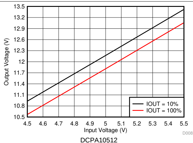
Figure 8. Line Regulation
