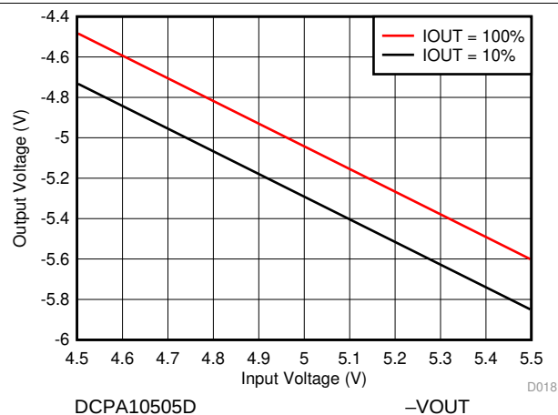
Figure 18. -VOUT Line Regulation
