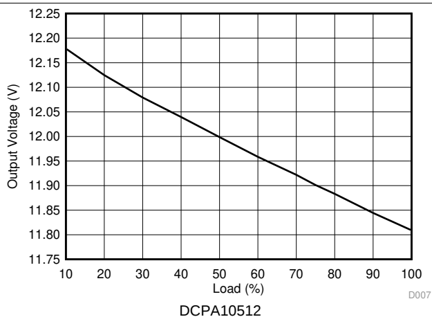
Figure 7. Load Regulation
