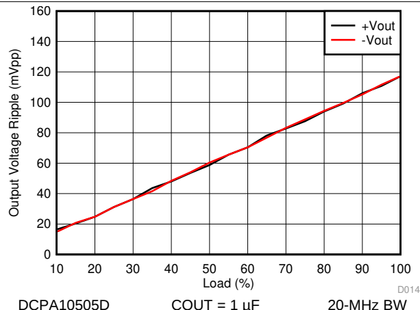
Figure 14. Output Ripple versus Load
