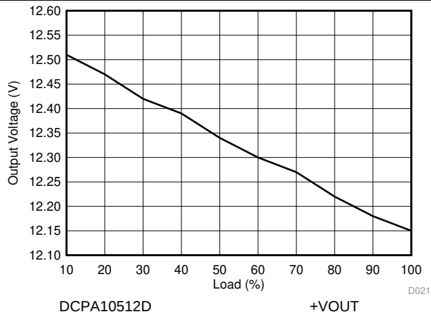
Figure 21. +VOUT Load Regulation
