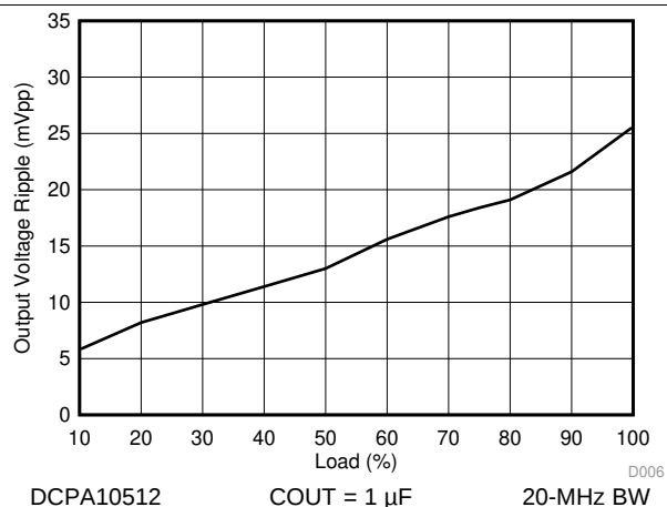
Figure 6. Output Ripple versus Load
