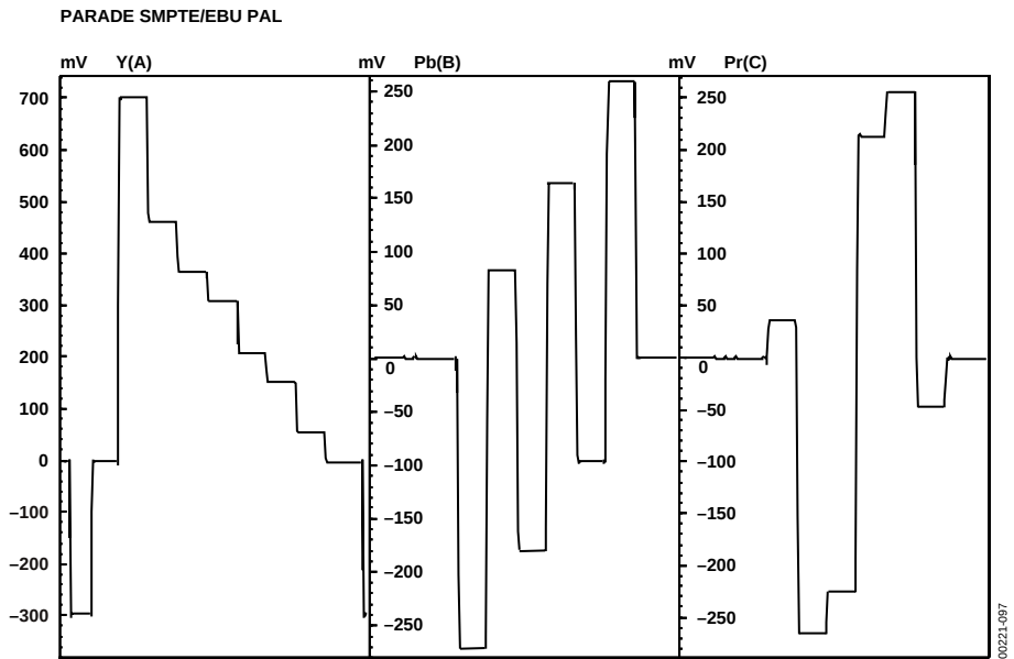
Figure 97. PAL YUV Parade Plot
