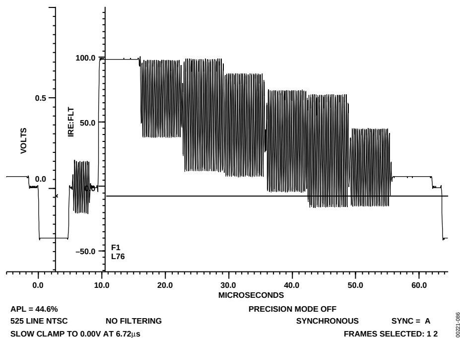
Figure 86. 100/7.5/75/7.5 NTSC Color Bars
