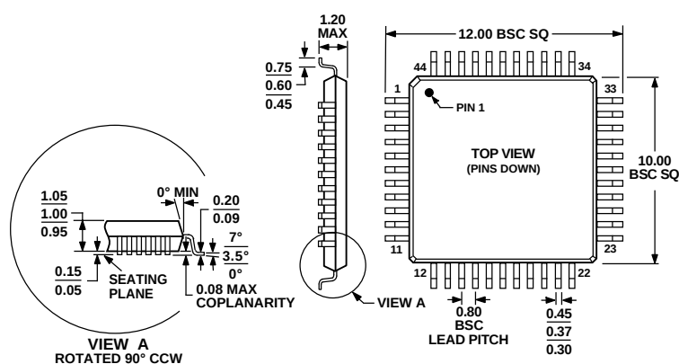
Figure 104. 44-Lead Thin Plastic Quad Flat Package [TQFP] (SU-44)
