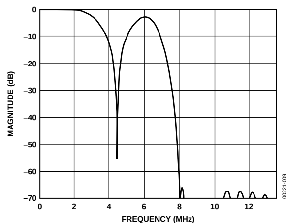
Figure 9. PAL Notch Luma Filter
