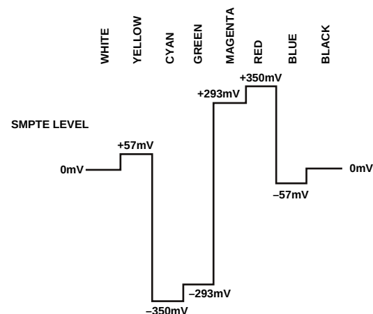
Figure 77. NTSC 100% Color Bars with Pedestal V Levels
