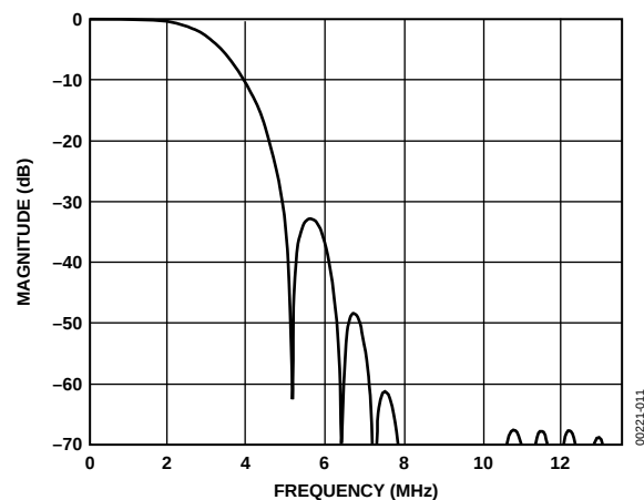
Figure 11. CIF Luma Filter
