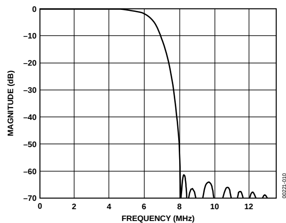
Figure 10. Extended Mode (SSAF) Luma Filter
