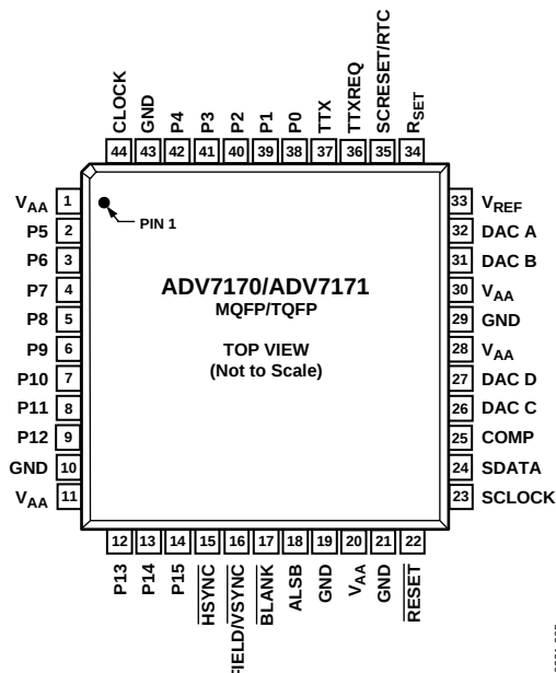
Figure 5. Pin Configuration
