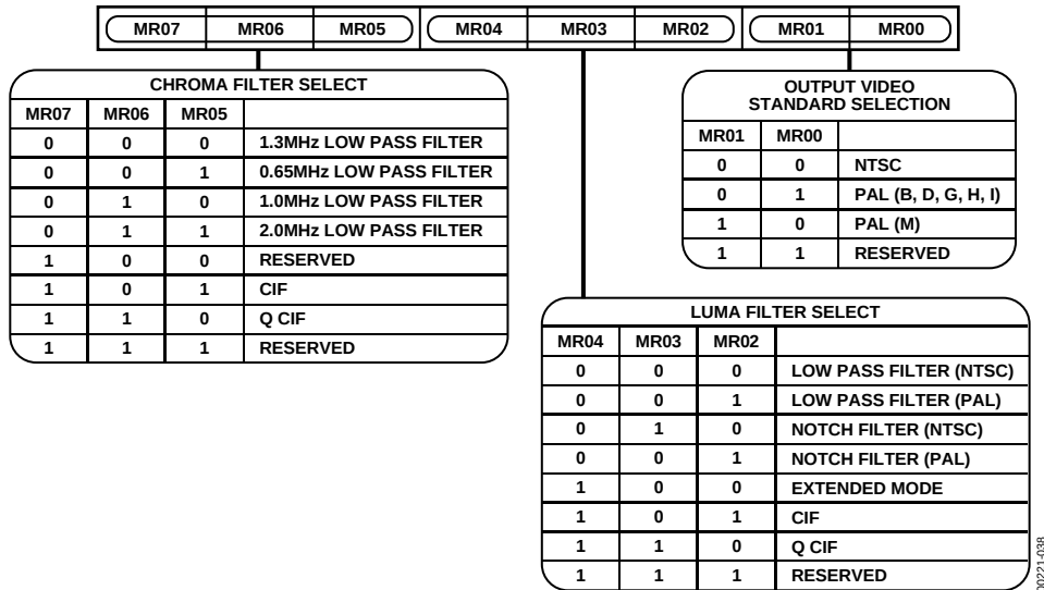
Figure 38. Mode Register 0
