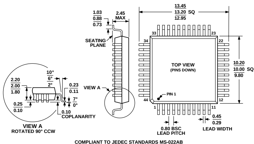
Figure 103. 44-Lead Metric Quad Flat Package [MQFP] (S-44-1)
