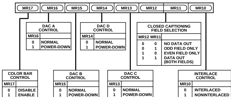
Figure 39. Mode Register 1
