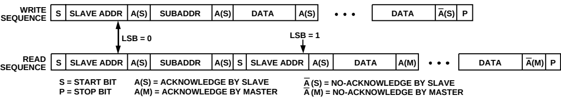
Figure 36. Write and Read Sequences
