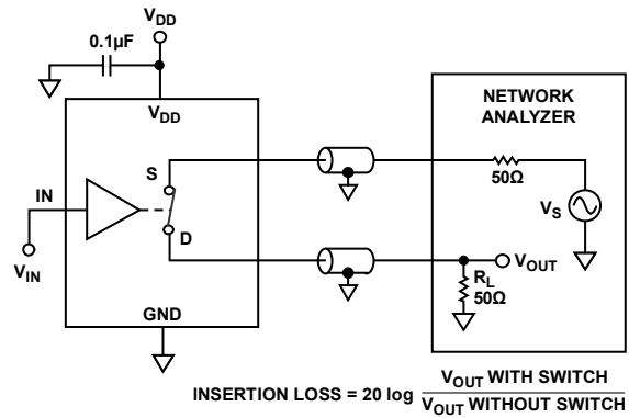
Figure 17. Bandwidth
