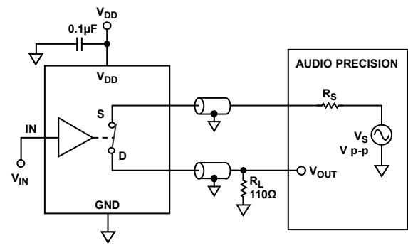
Figure 18. THD + Noise
