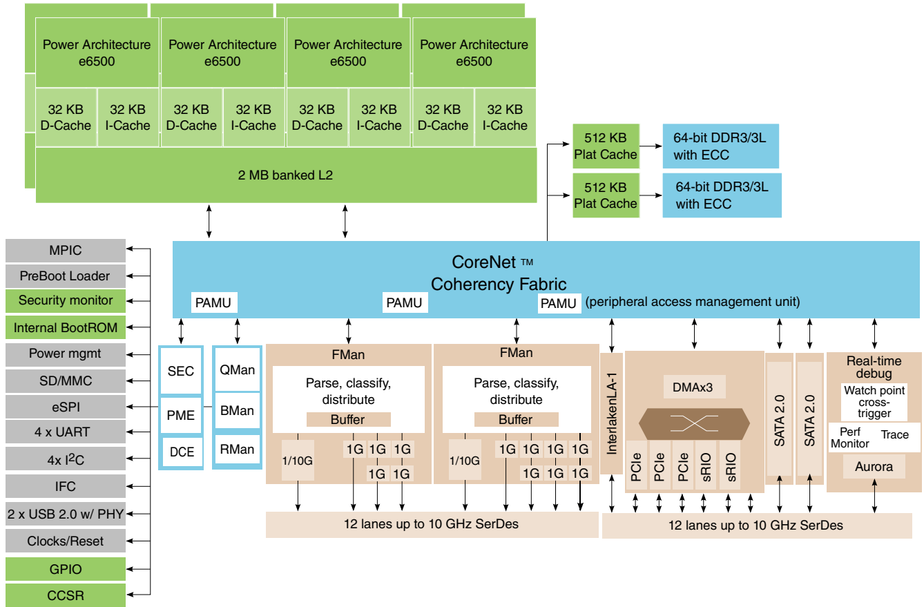
Figure A-1. T4160 block diagram
