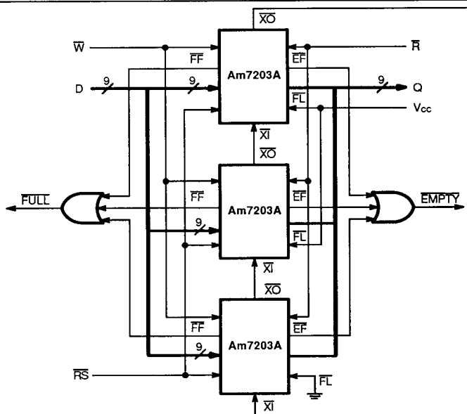
Figure 14. Depth-Expansion to Form 6,144 x 9 FIFO
