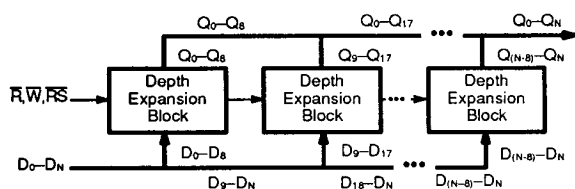
Figure 14. Depth-Expansion to Form 6,144 x 9 FIFO
