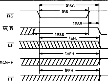
Figure 2. Reset Timing 15492B-5
