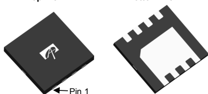
DFN 3.3x3.3 EP Top View Bottom View
