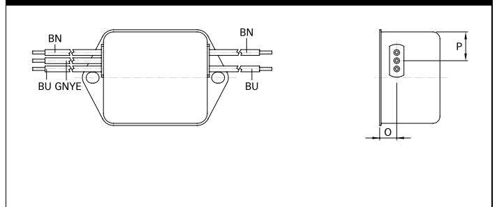
Connection style -07, 16 A types (same dimensions as style -06)
