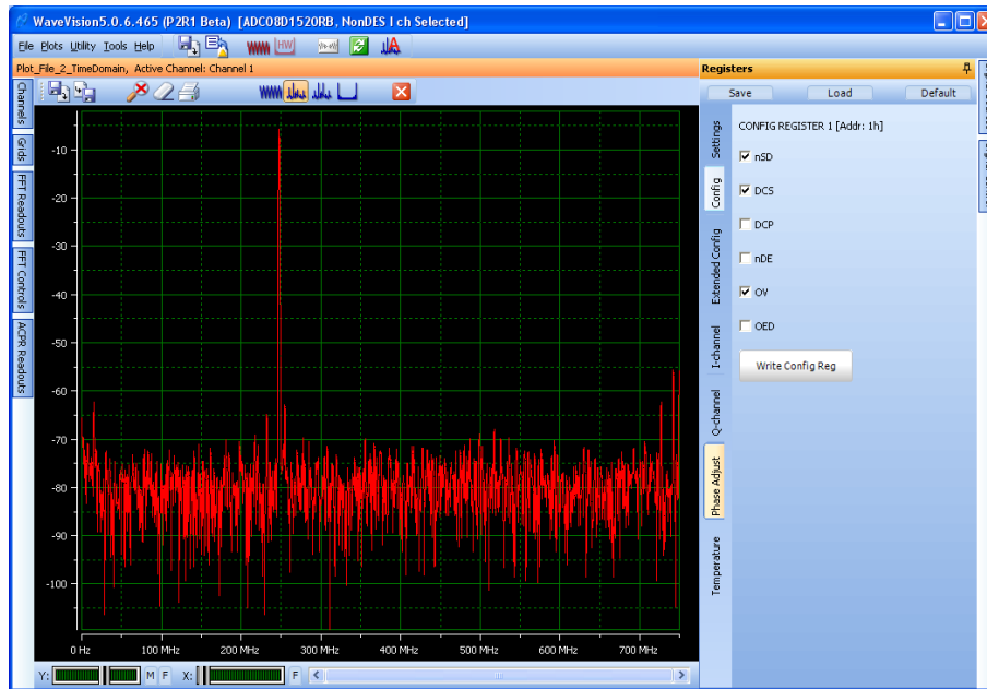
Figure 10: Config Panel
