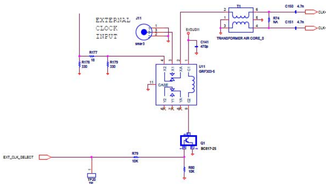
Figure 15. External / internal clock selection circuit on ADC08D1520RB
