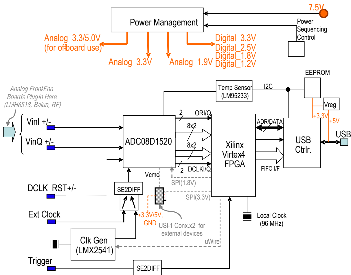
Figure 16: ADC08D1520RB System Block Diagram
