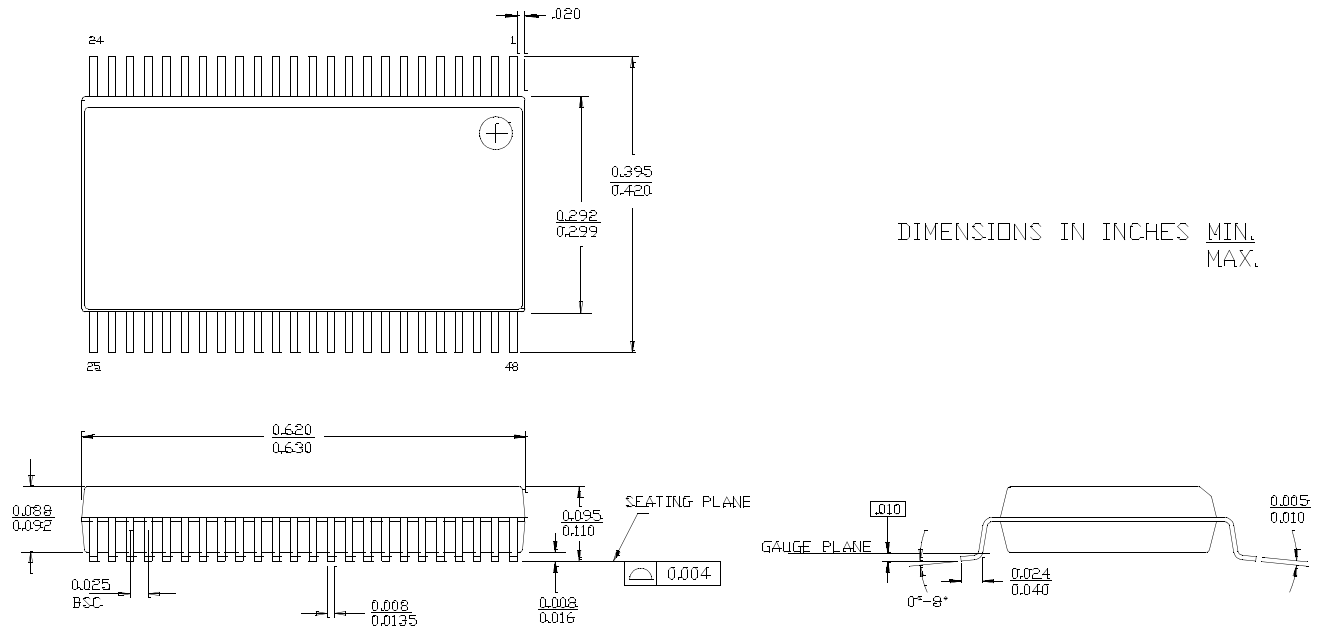
Figure 17. 48-Pin Shrunk Small Outline Package (51-85061)
