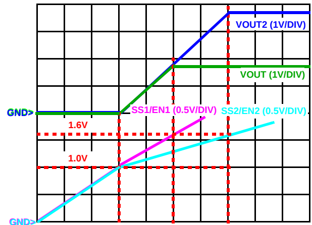
FIGURE 6. VOLTAGE TRACKING
