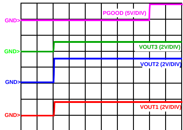
FIGURE 9. PGOOD DELAY
