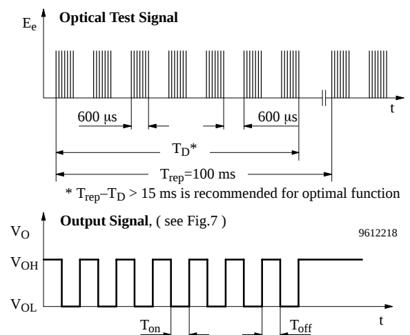
Figure 6. Output Function
