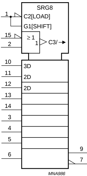
Fig.3 Logic symbol (IEEE/IEC).
