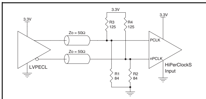
Figure 2C. HiPerClockS PCLK/ \overline{\text{PCLK}} Input Driven by a 3.3V LVPECL Driver
