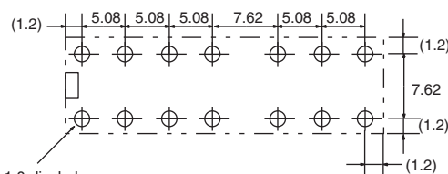
Terminal Arrangement/ Internal Connections (Bottom View)
