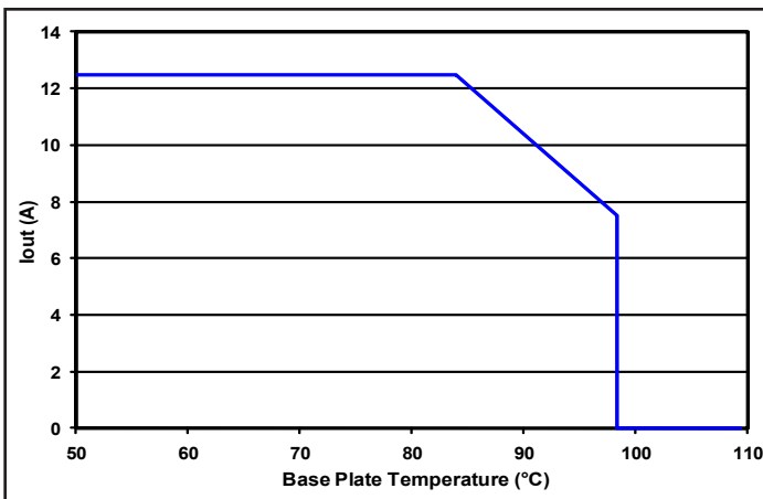
Figure 3: Encased converter max. output power derating vs. base plate temperature (nominal input voltage).
