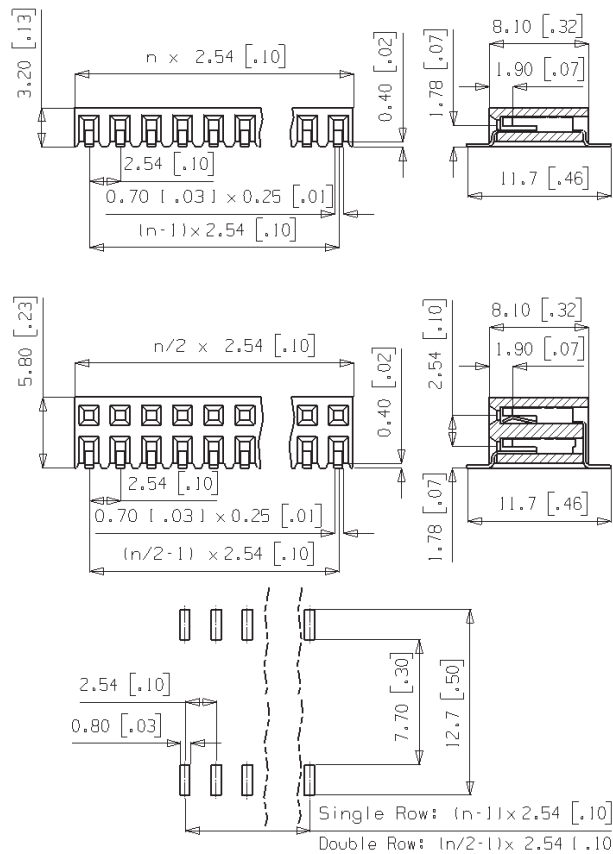
PCB Layout
