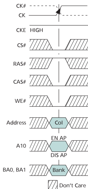
Figure 19: WRITE Command
