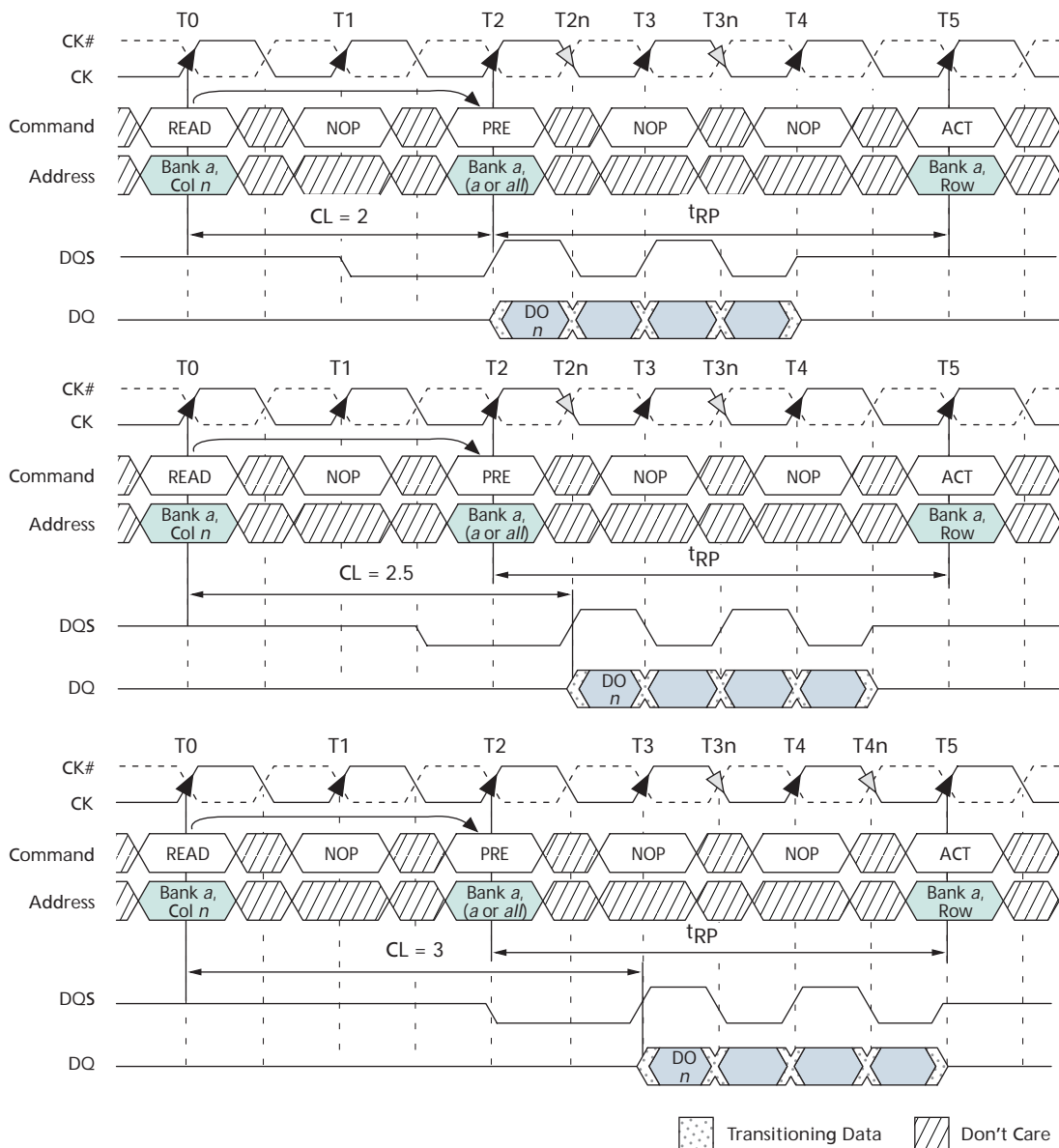
Figure 33: READ-to-PRECHARGE
