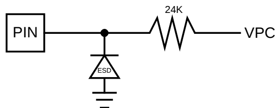
Figure 11: On_Off Pin
