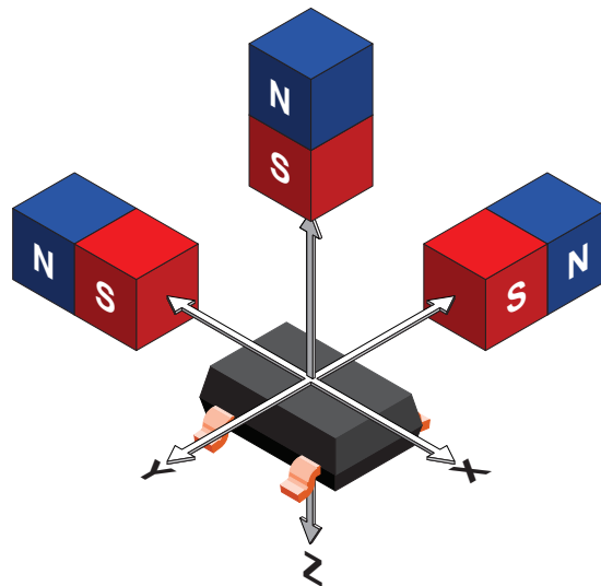
Figure 1: Three Dimensions of Magnet Orientation. Applied field may be either north or south polarity.
