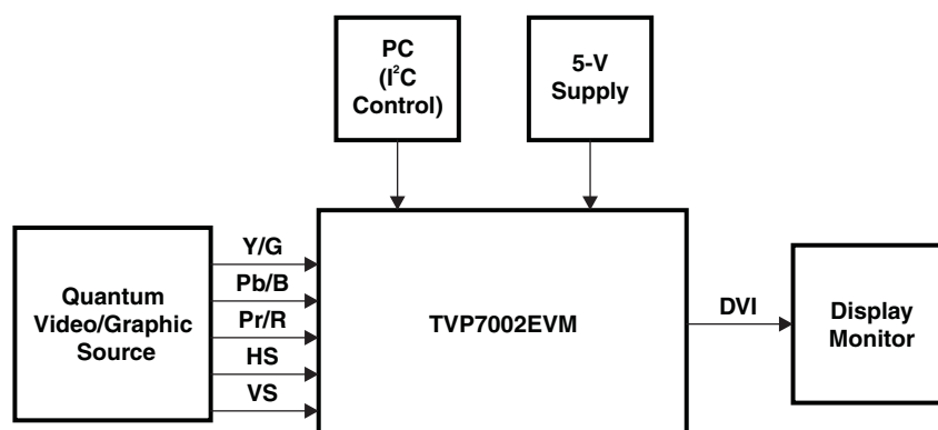
Figure 1-2. TVP7002EVM System Level Block Diagram
