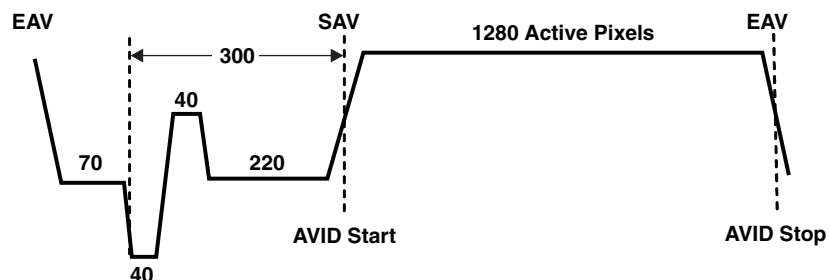
Figure B-1. 720p60 Example, Total Line Length = 1650 Pixels
