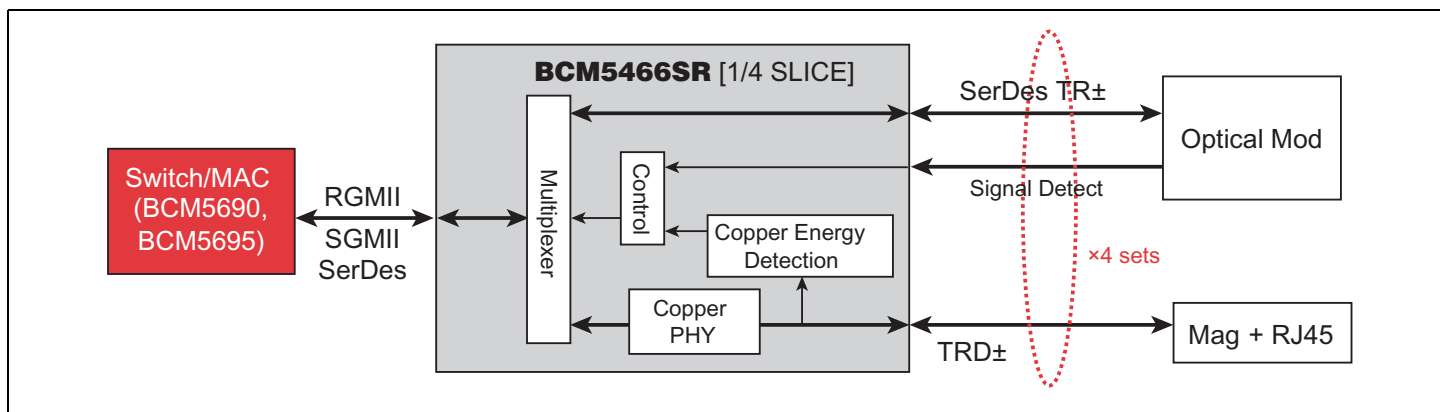
BCM5466SR System Diagram
