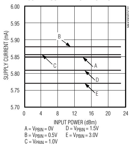
SUPPLY CURRENT vs. INPUT POWER
