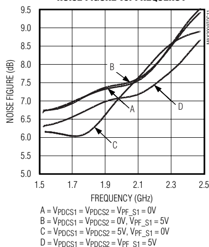
NOISE FIGURE vs. FREQUENCY
