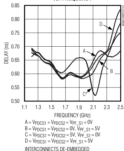
GROUP DELAY vs. FREQUENCY
