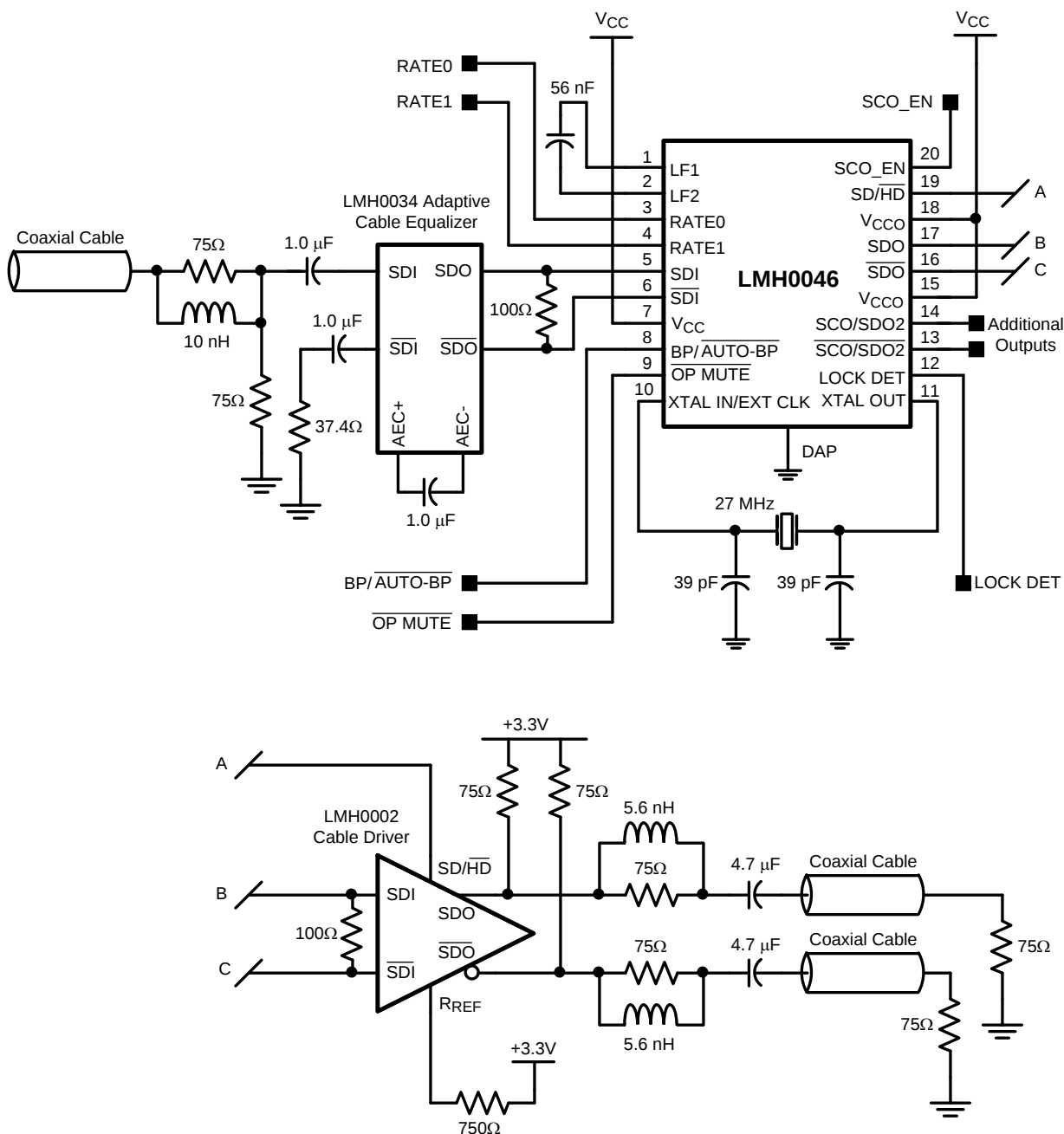
Figure 7. Application Circuit
