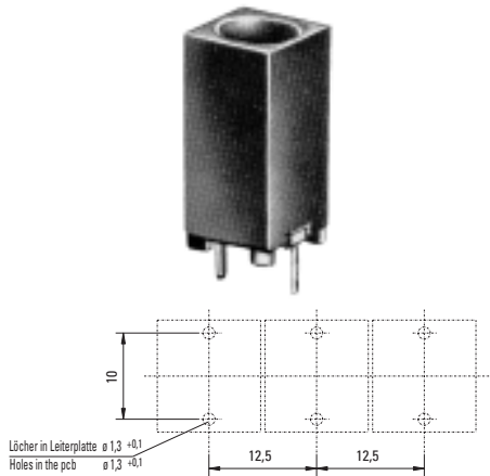
Holes in the Printed Circuit Board
