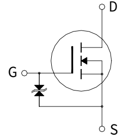
SCHEMATIC DRAWING
