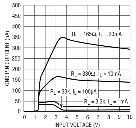
GND Pin Current LT3008-3.3
