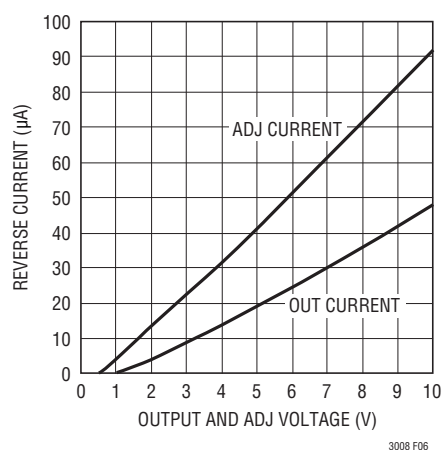
Figure 6. Reverse-Output Current
