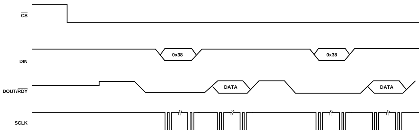
Figure 14. Continuous Conversion
