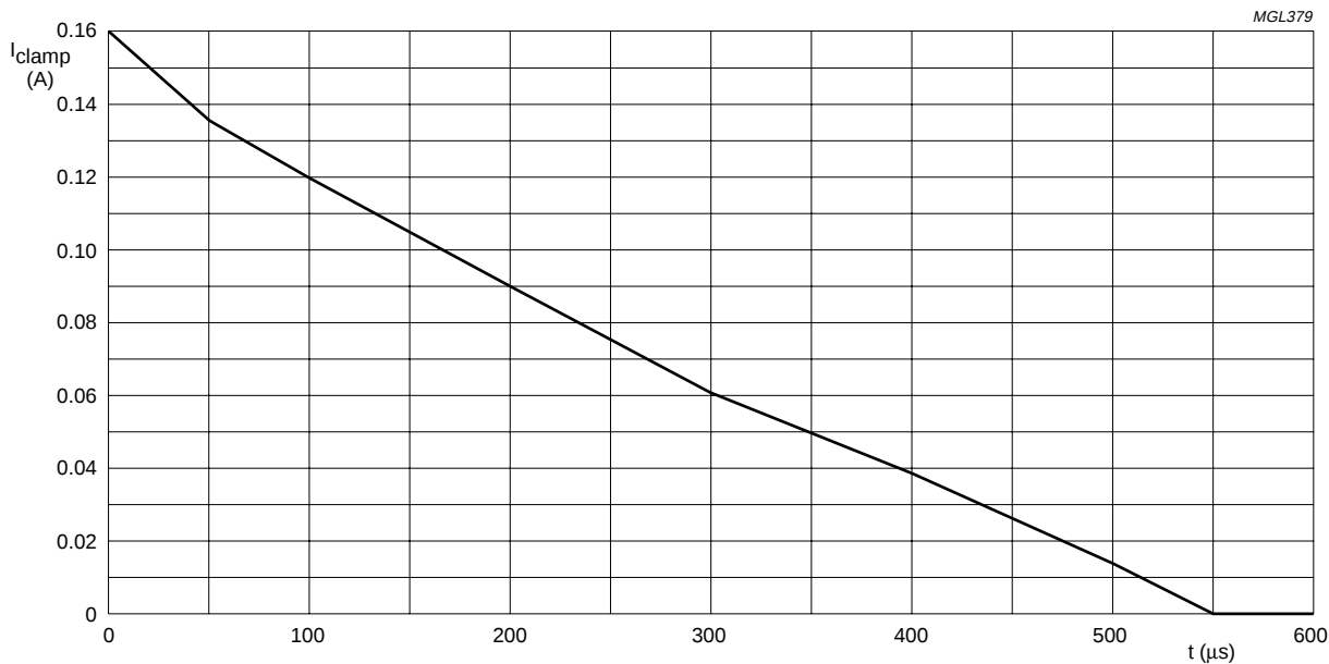
Fig.5 Maximum current during inductive turn-off ( T_{amb} = 85^{\circ}C ).
