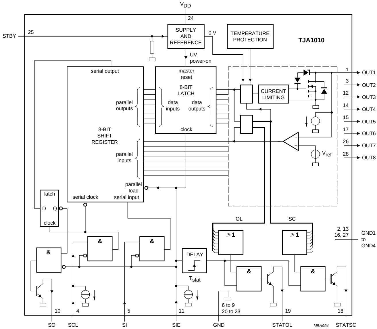
Fig.1 Block diagram.
