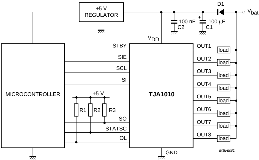
Fig.7 Application example.
