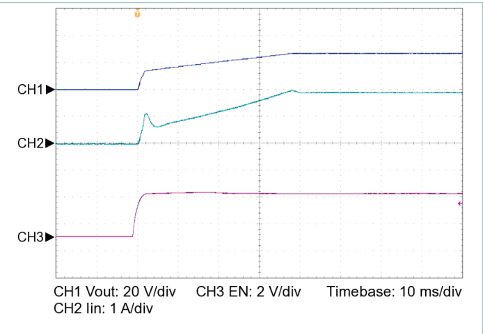
Figure 17 — Startup from EN, V_{IN} = 270\text{ V} , C_{OUT\_EXT} = 2000\text{ μF} , R_{LOAD} = 1.568\text{ Ω}
